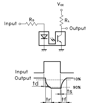
Test Circuit for Response Time
