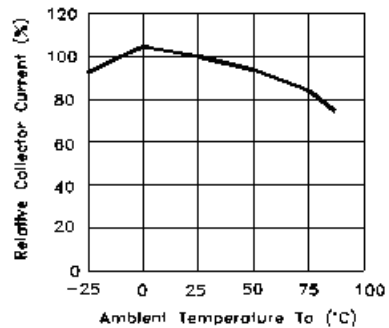
Fig.4 Collector Current vs. Ambient Temperature
